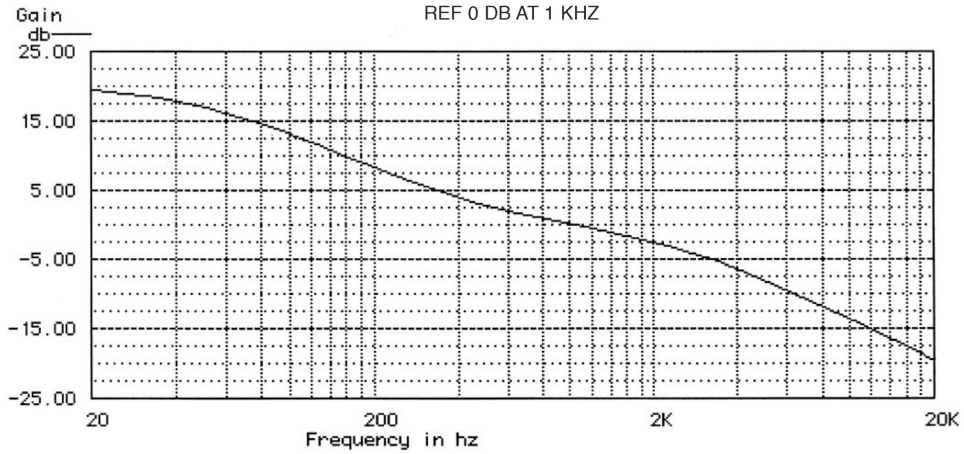
RIAA REPRODUCE EQUALIZATION REF 0 DB AT 1 KHZ
