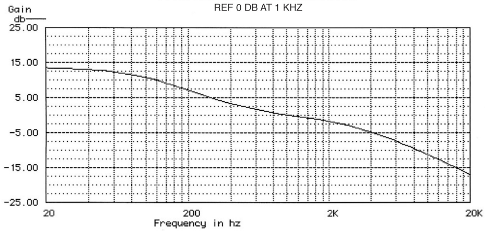
FFRR REPRODUCE EQUALIZATION REF 0 DB AT 1 KHZ
